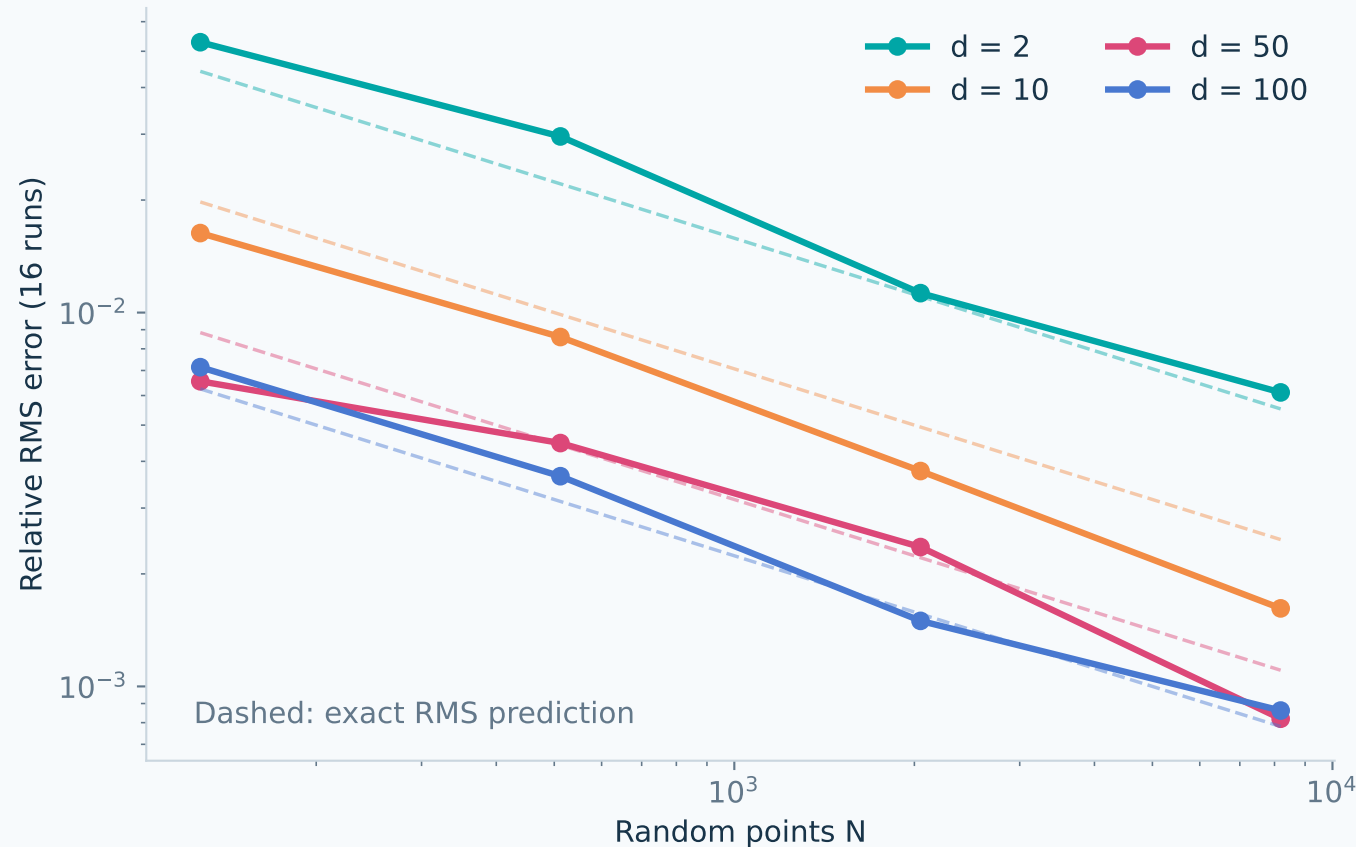
Energy integration: measured error vs. theory
